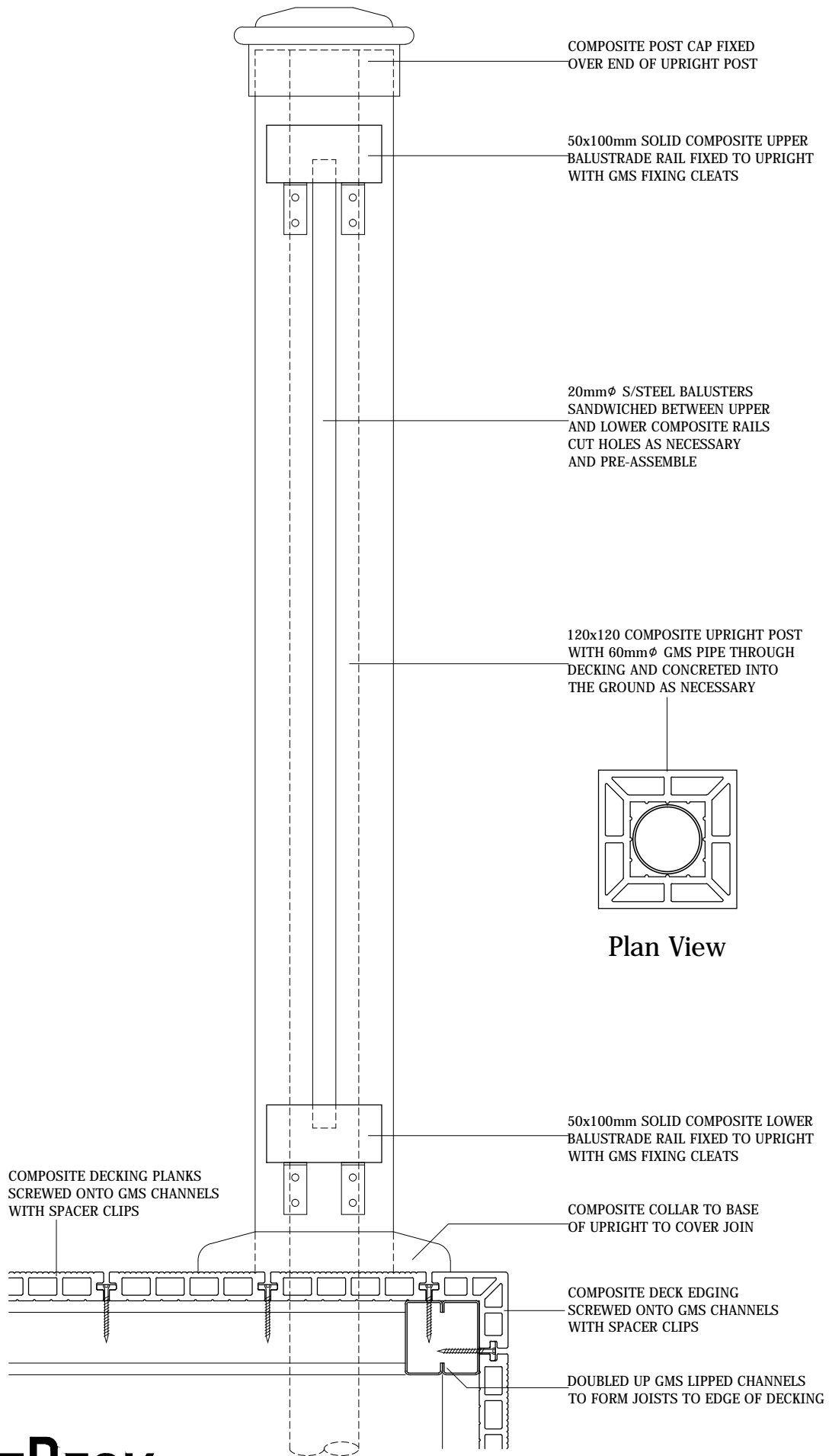
TYPICAL BALUSTRADE DETAIL Scale 1:5 - Composite and S/Steel Components
